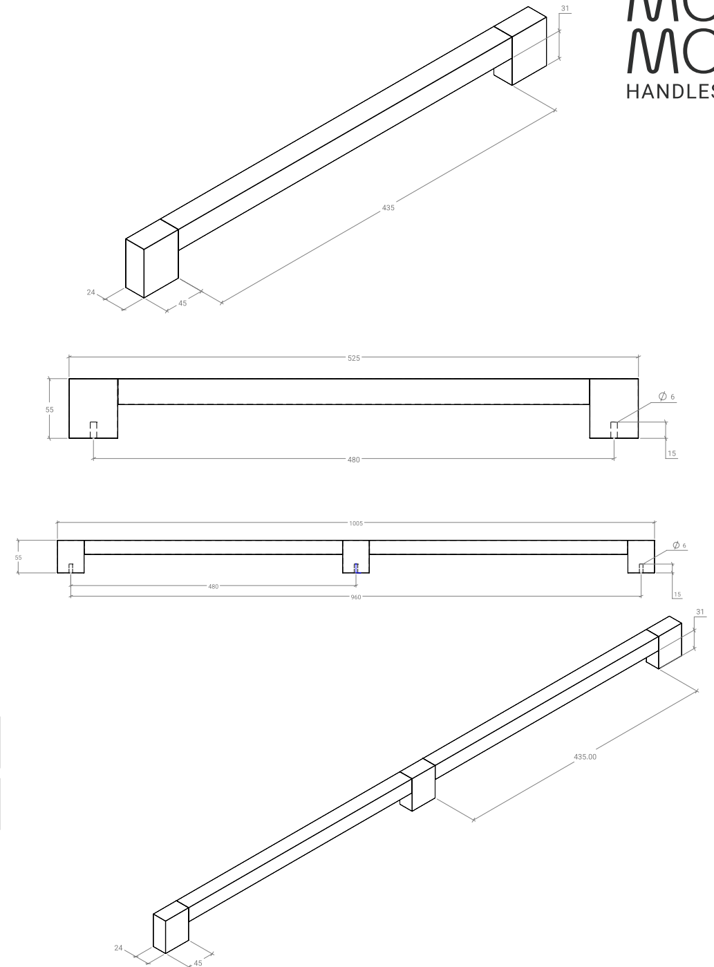
D Handle
