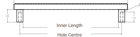
Bar Handle
